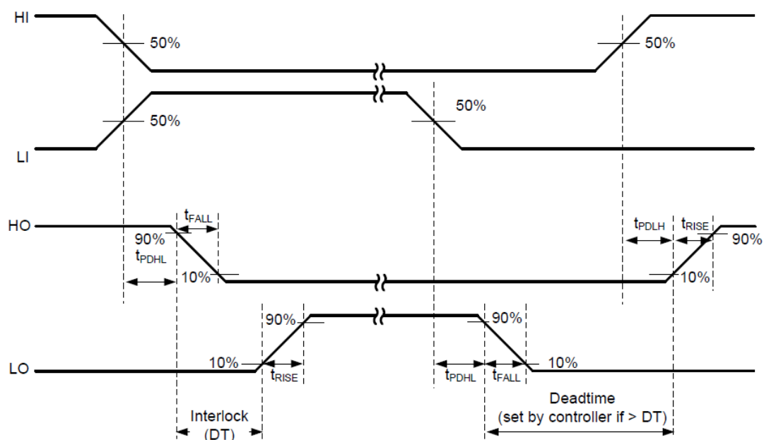
Figure 1. Typical Test Timing Diagram
