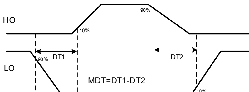
Figure 2. Dead-time matching
