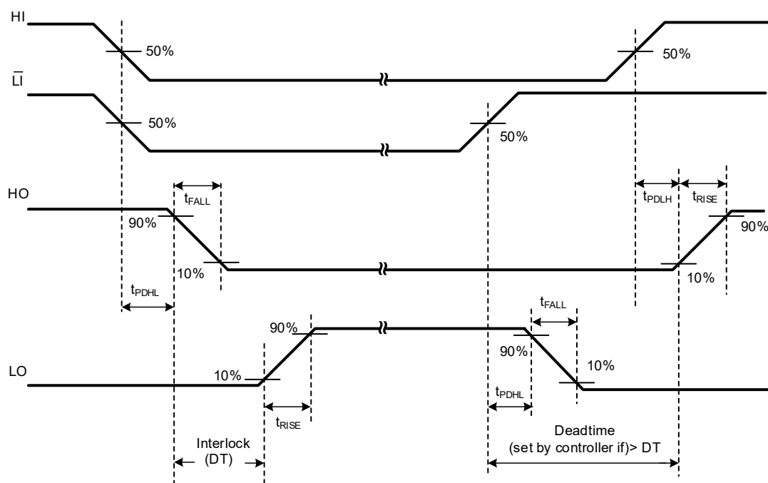
Figure 1. Typical Test Timing Diagram
