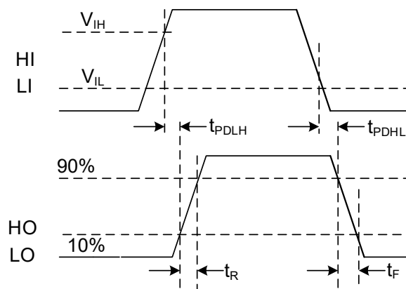
Figure 1. Switching Time Waveform Definitions
