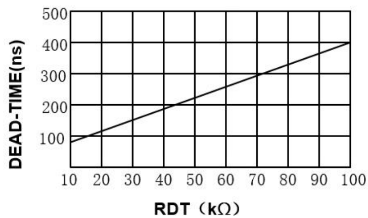
Figure 4. Dead-Time vs RDT Resistor Value
