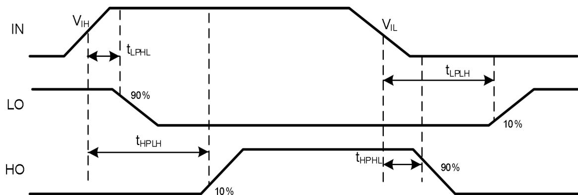
Figure 1. Typical Test Timing Diagram
