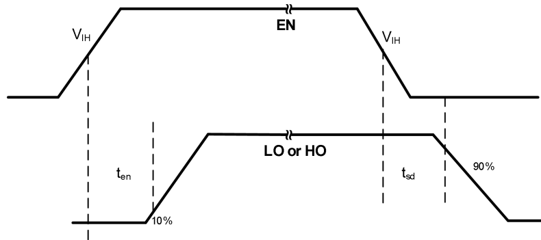
Figure 3. CFG2216 Enable
