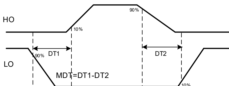
Figure 2. Dead-time Waveform Definitions
