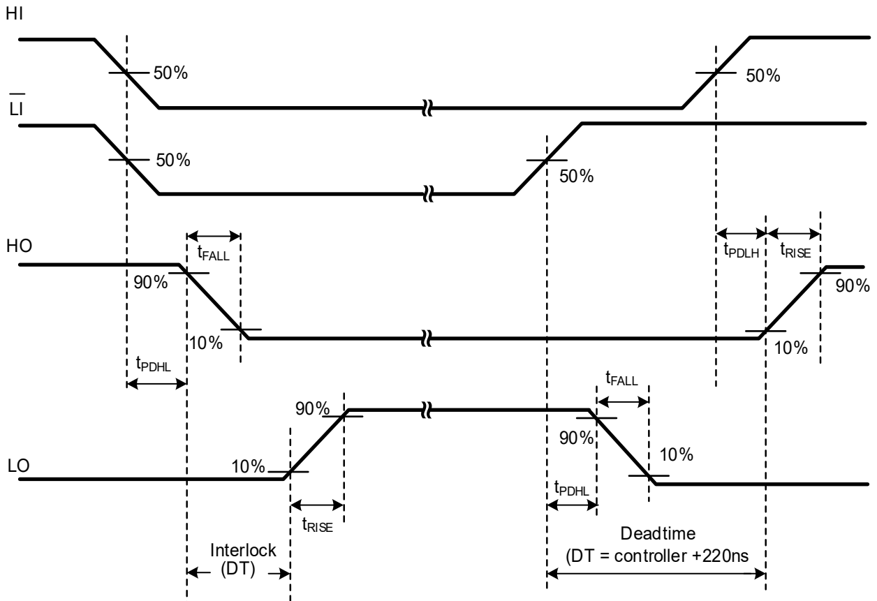
Figure 1. Switching Time Waveform Definitions
